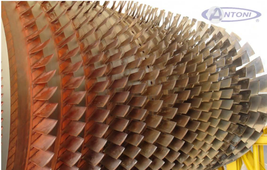
Turbine Rotor
